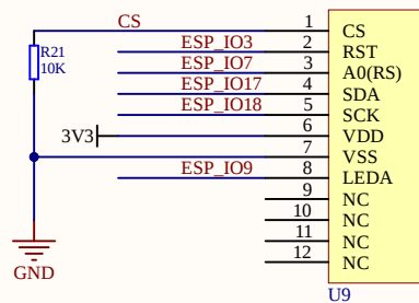
JLX240-00302 屏幕接口, 排母2.54*12P
